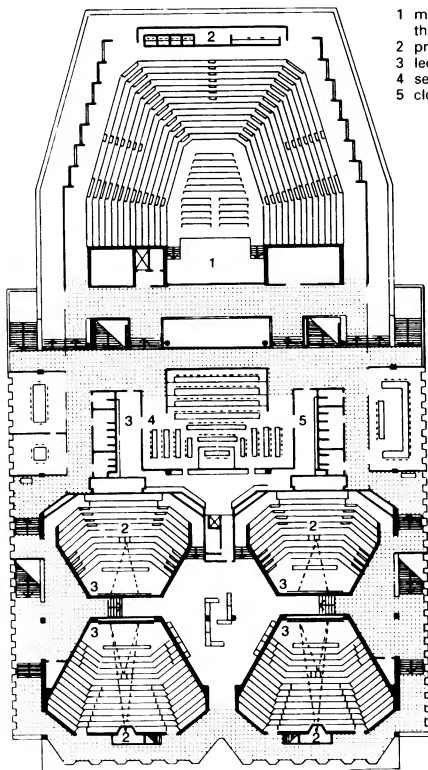
③ Lecture theatre at the TH Delft
